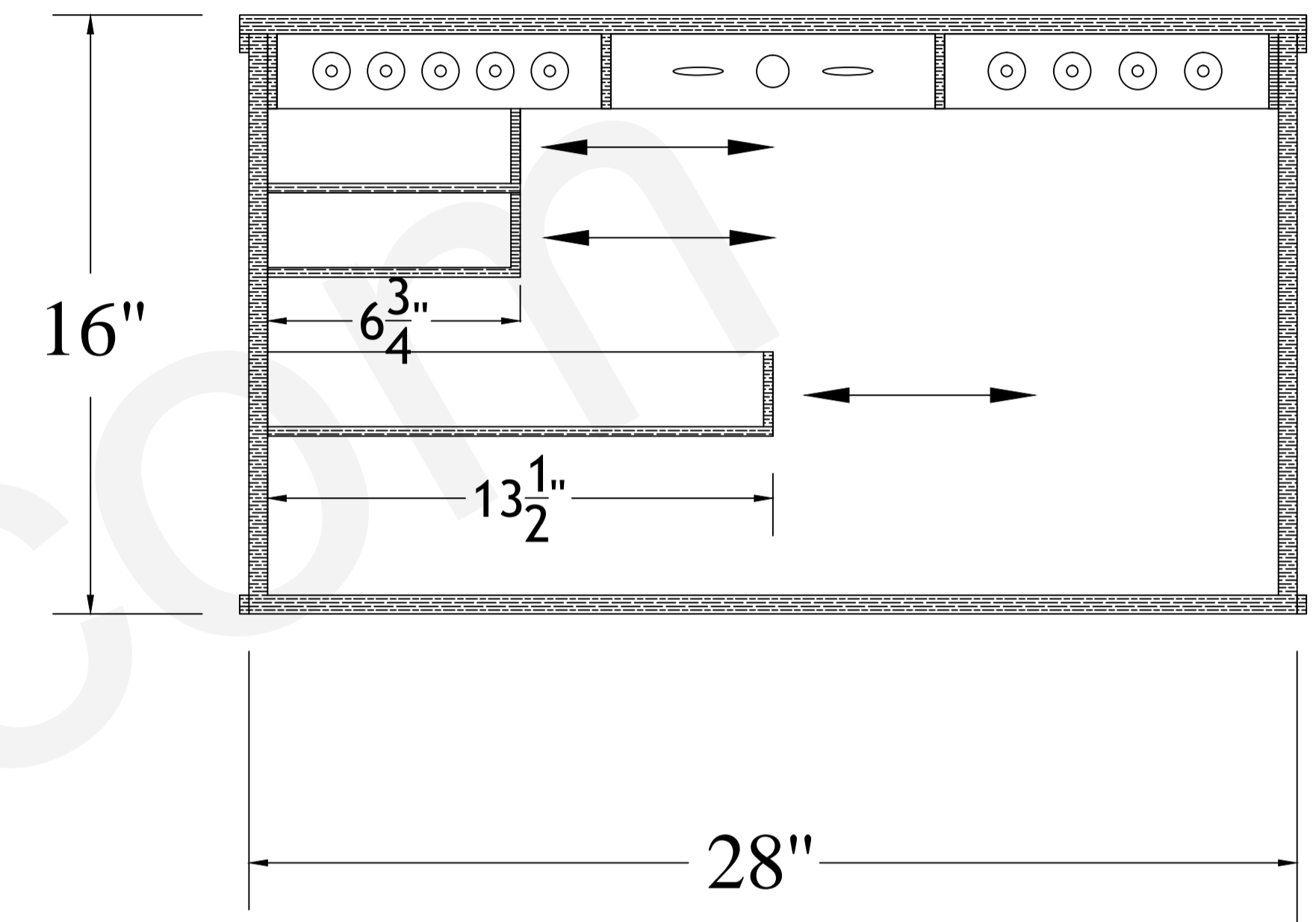
SECTION X-X
