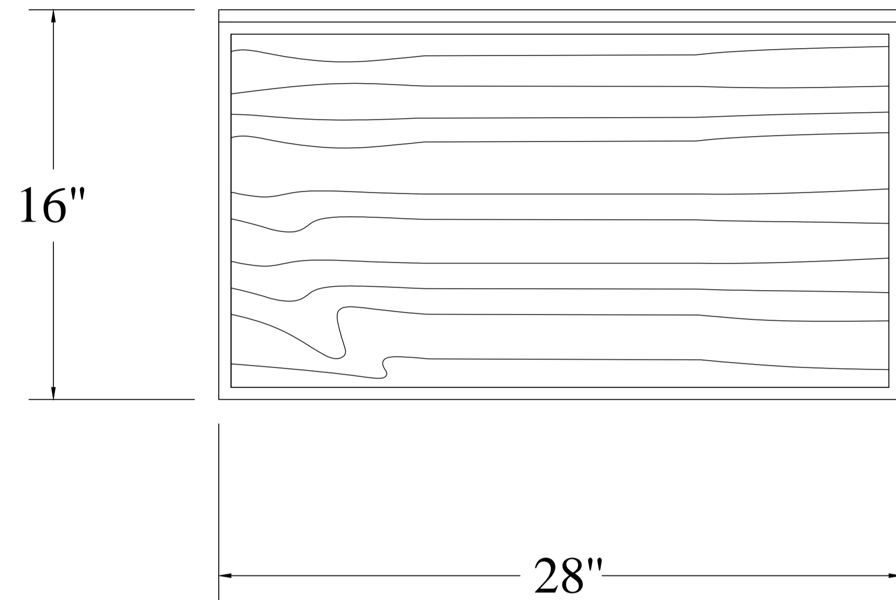
FRONT VIEW
